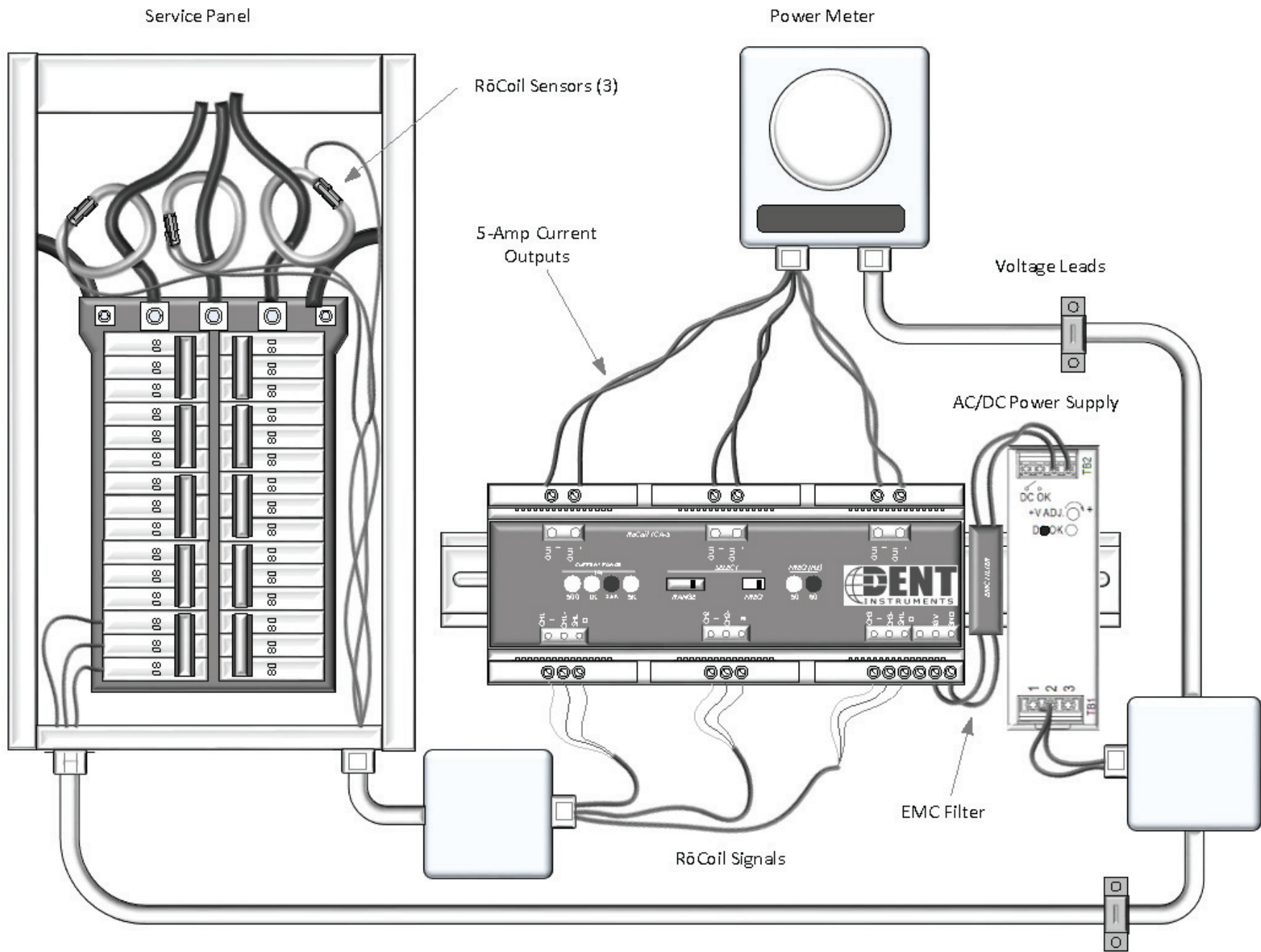
Figure 2-1: Recommended Installation
